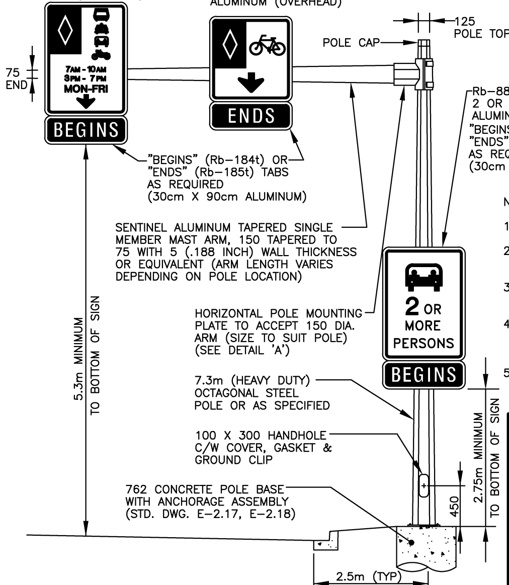
CANTILEVER SIGNS & POLE ASSEMBLY
