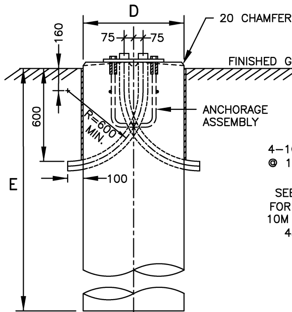
ELEVATION LAYOUT
