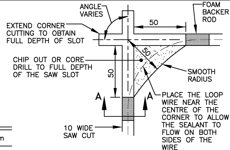
DETAIL AT 90° BEND
