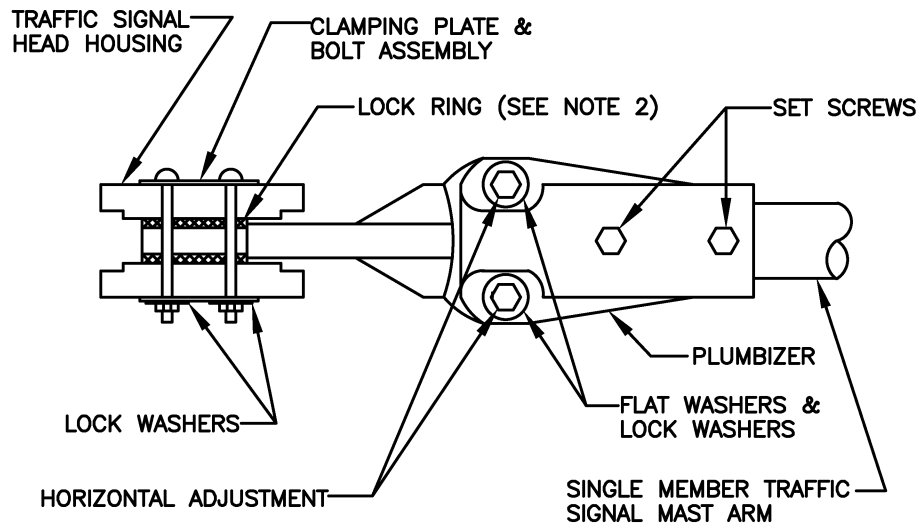
PLUMBIZER ATTACHMENT
