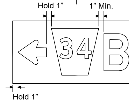
End Spacing Detail Unconstrained
