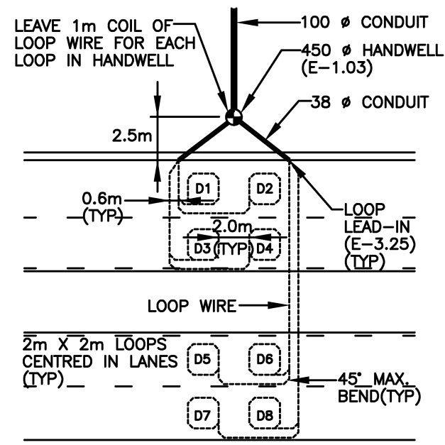
5 LANE CONFIGURATION
