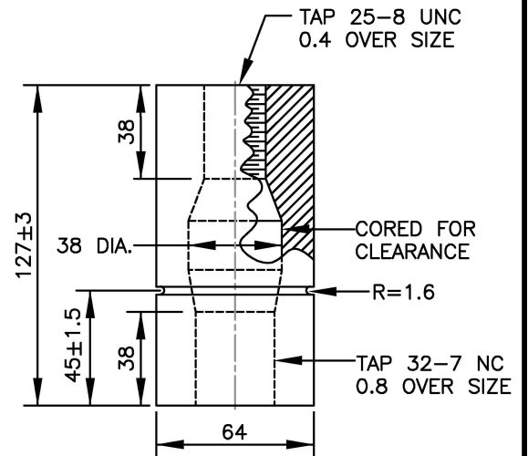
STANDARD GROOVED COUPLER DETAIL
