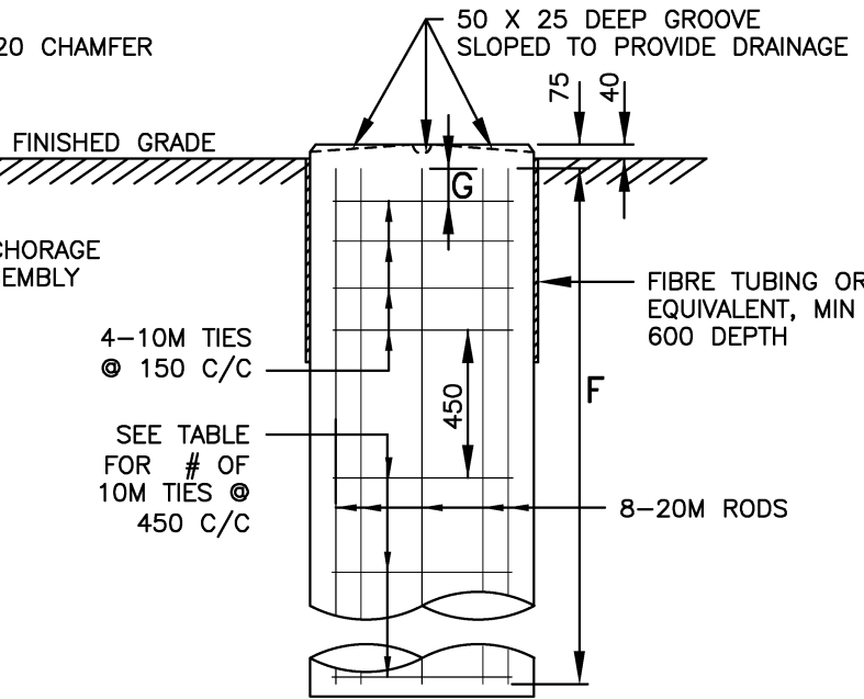
ELEVATION REINFORCEMENT
