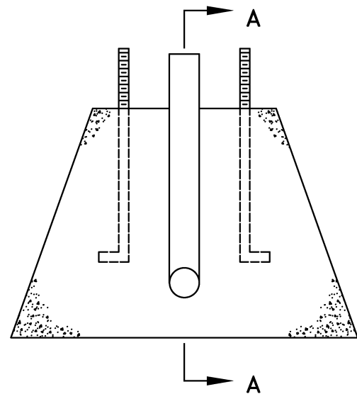
RIGHT VIEW
