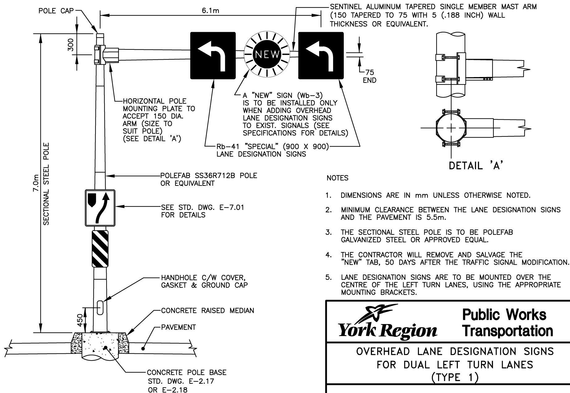
CANTILEVER SIGN & POLE ASSEMBLY
