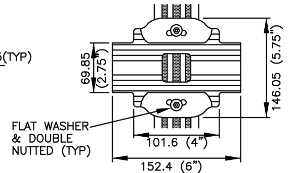
ALUMINUM CASTING DETAIL
