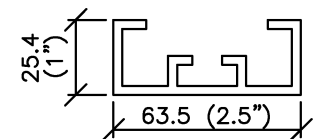
SECTION A-A ALUMINUM EXTRUSION DETAIL
