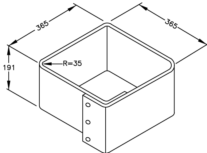
SHROUD COVER
