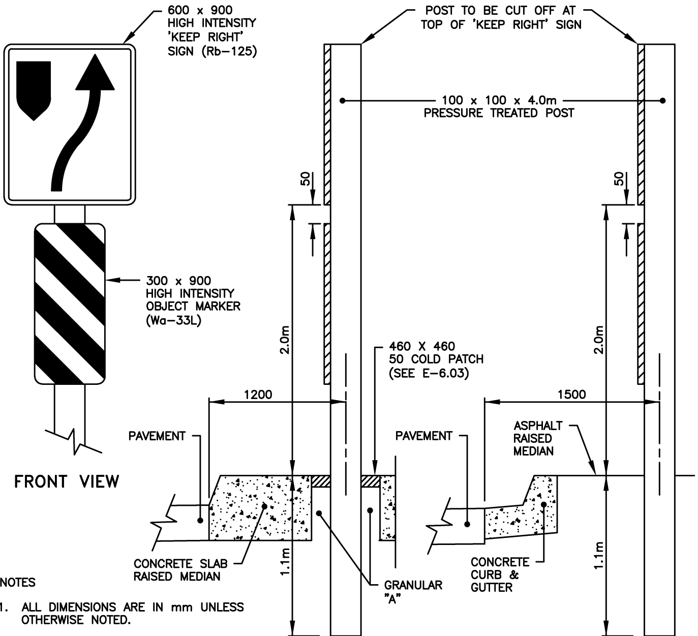
CONCRETE SLAB RAISED MEDIAN
